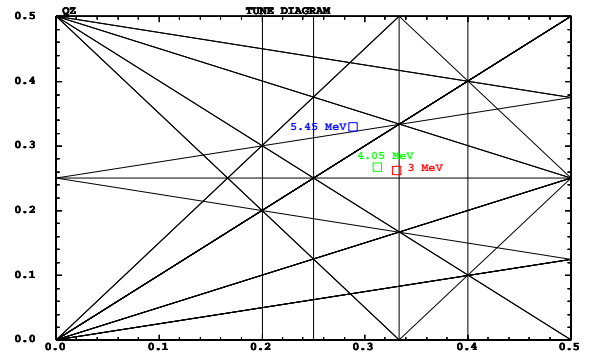
FIG. 11 – Left : 2-D motion (x, x') , 1000-cell stability limits, at 0.05 cm precision in x , at 3, 4.05, 5.45 MeV. No fringe fields. Pure (larger amplitude) and coupled (smaller amplitude) motion in the presence of a very small z component. Right : tunes per cell corresponding to coupled stability limits in the tune diagram; systematic resonances up to the fifth order.
